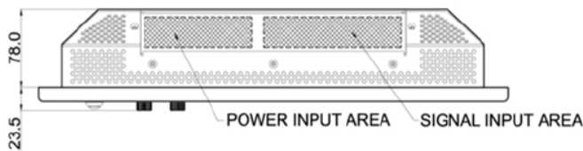
BOTTOM VIEW
